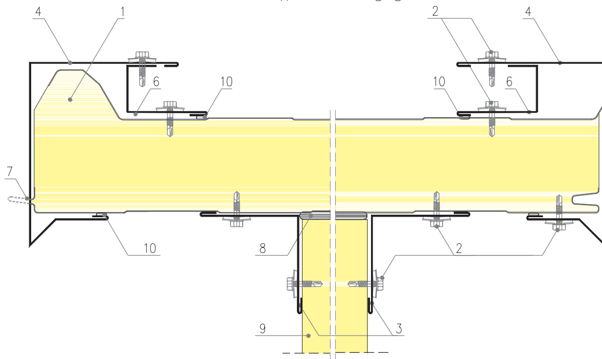
Type I - overhanging
