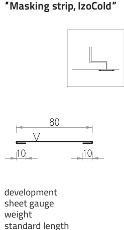
Drawing 59. Ob-23 flashing "Masking strip, IzoCold"
