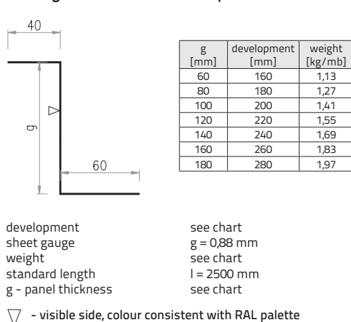
Drawing 74. L-04 fastener "Z strip"
