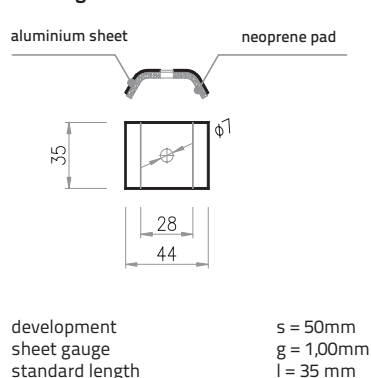
Drawing 73. L-03 fastener "Saddle washer"
