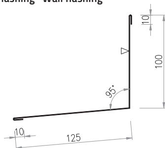
Drawing 54. Ob-17 flashing "Wall flashing"
