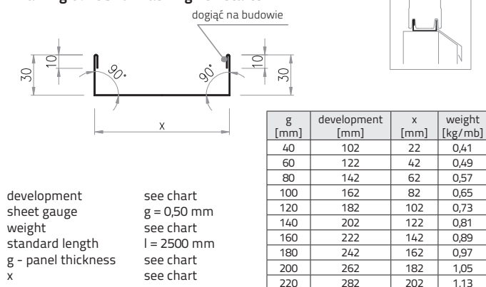
Drawing 67. Ob-41 flashing "C2 starter"
