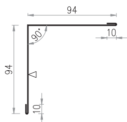
Drawing 46. Ob-09 flashing "Large inner corner"
