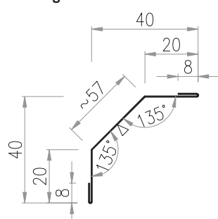
Drawing 52. Ob-15 flashing "Broken inner corner"
