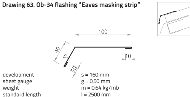
Drawing 63. Ob-34 flashing "Eaves masking strip"
