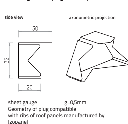
Drawing 75. Rib plug for roof panel "Z1"
