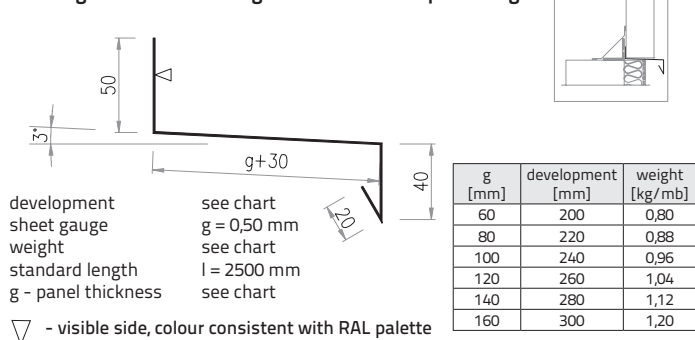
Drawing 71. Ob-45 flashing "Substructure drip flashing"
