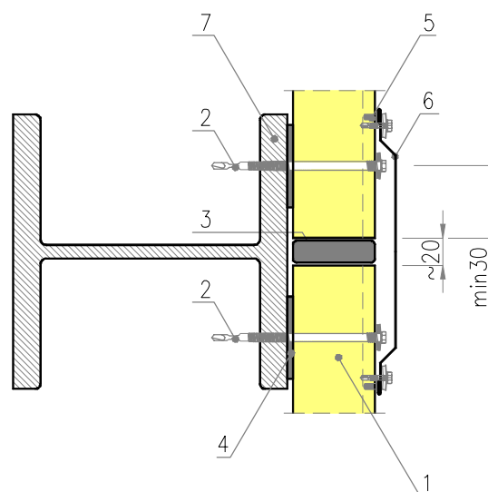
PANEL JOINT
