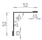
Drawing 48. Ob-11 flashing "Small inner corner"
