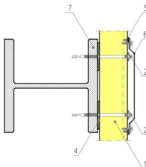
INTERMEDIATE SUPPORT
