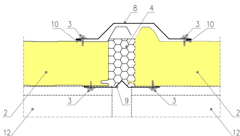
Sliding joint - roof
