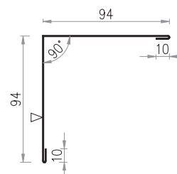
Drawing 47. Ob-10 flashing "Large outer corner"
