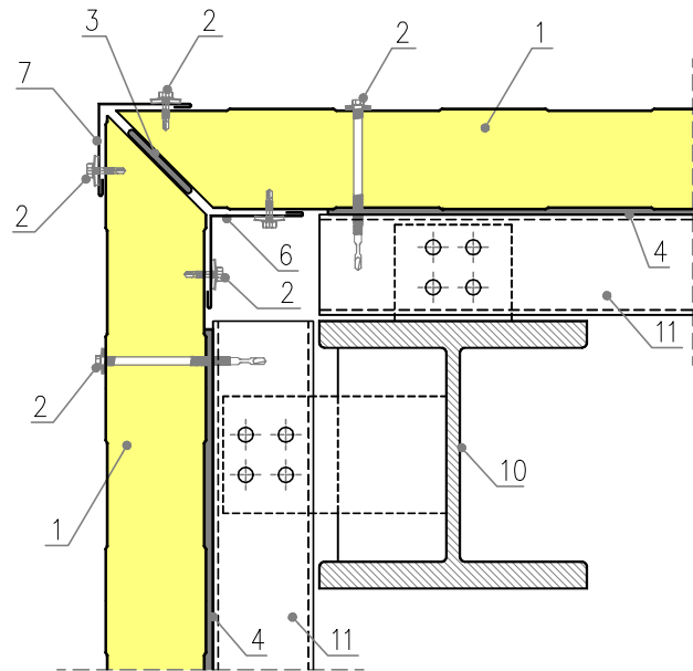
Type II - vertical arrangement
