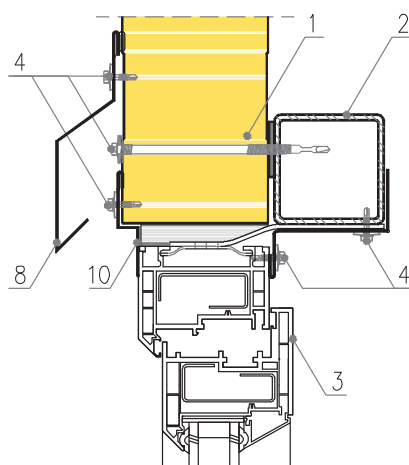
Horizontal edge of window – flashings
