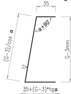
Drawing 56. Ob-19 flashing "Gutter downside flashing"
