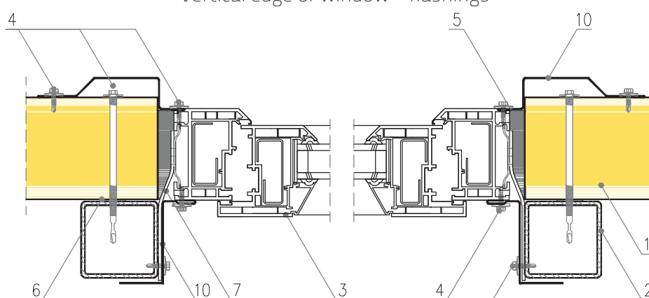
Vertical edge of window – flashings
