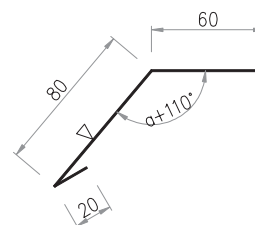
Drawing 55. Ob-18 flashing "Gutter flashing for Ob-19"
