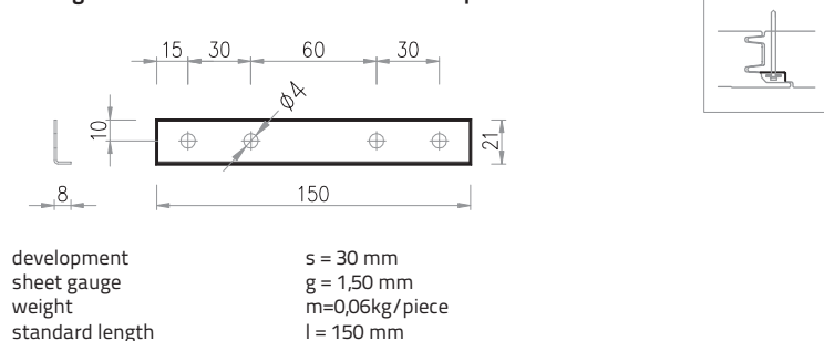
Drawing 72. L-02 fastener "IzoGold PIR/PIR+ panel connector"
