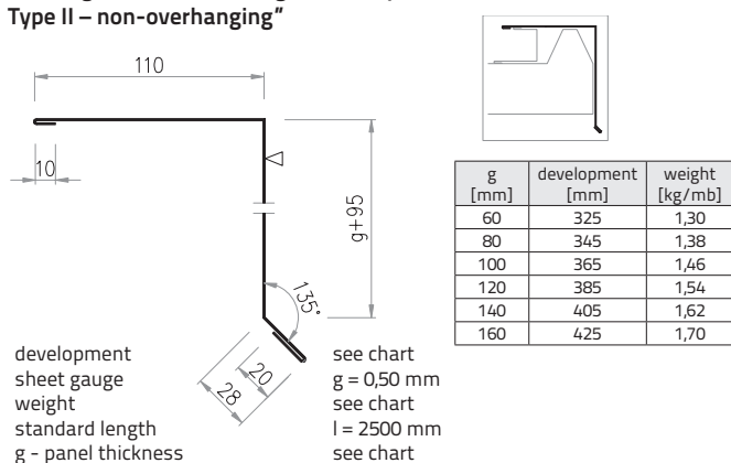
Drawing 61. Ob-32 flashing "IzoRoof panel wind beam, Type II – non-overhanging"
