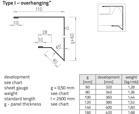
Drawing 60. Ob-31 flashing "IzoRoof panel wind beam, Type I – overhanging"
