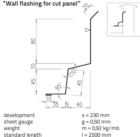
Drawing 58. Ob-22 flashing "Wall flashing for cut panel"
