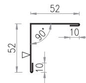
Drawing 49. Ob-12 flashing "Small outer corner"
