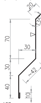
Drawing 53. Ob-16 flashing "Drip cap strip"
