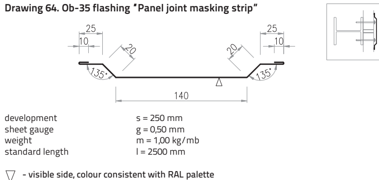
Drawing 64. Ob-35 flashing "Panel joint masking strip"
