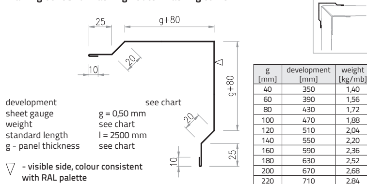
Drawing 68. Ob-42 flashing "Outer masking corner"
