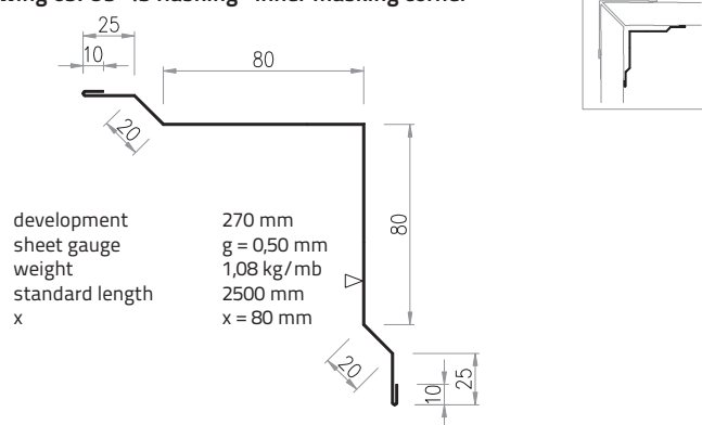
Drawing 69. Ob-43 flashing "Inner masking corner"
