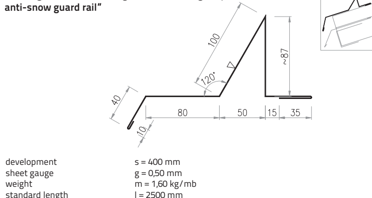
Drawing 62. Ob-33 flashing "Eaves masking strip with anti-snow guard rail"
