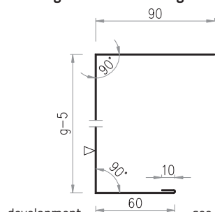
Drawing 50. Ob-13 flashing "Gutter downside flashing"
