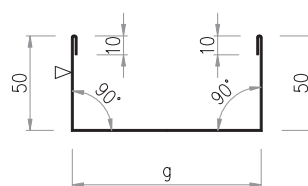
Drawing 57. Ob-20 flashing "C1 starter"
