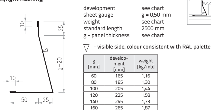
Drawing 70. Ob-44 flashing "Inner skylight flashing"
