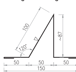
Drawing 51. Ob-14 flashing "Anti-snow guard rail"
